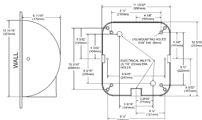
Model XL-SB Surface-mounted, Automatic, Brushed Stainless Steel Cover
