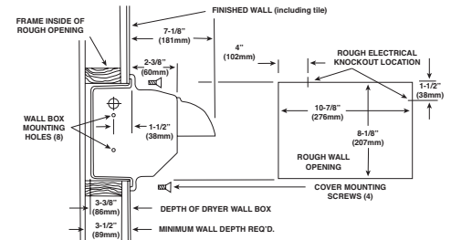
PART #R76-IC
