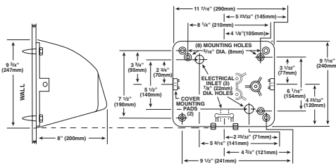
PART #HO-IC
